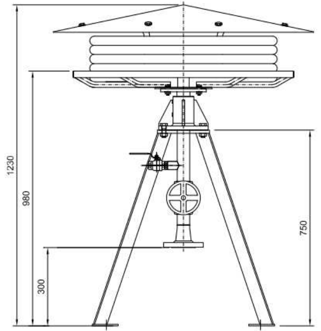
( LIVE HOSE REEL DIMENSIONS)
